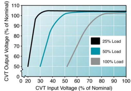
Figure 3. As the CVT load increases, the ability of the CVT to regulate its output voltage decreases.
