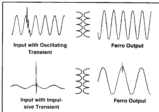
Figure 8. CVT output responses to input voltages with oscillating and impulsive transients.
