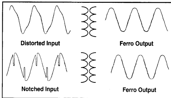
Figure 7. CVT output voltage with distorted and notched input voltages at full load.
